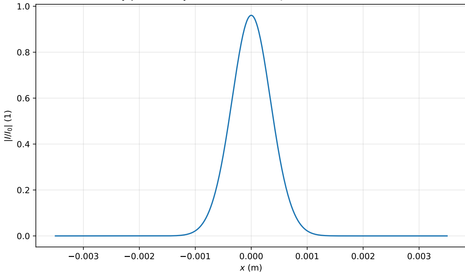
Intensity profile I(x, y = 0, z = 0.637m)/I_0 , P_{in}=0.2P_{cr} , artificial time
